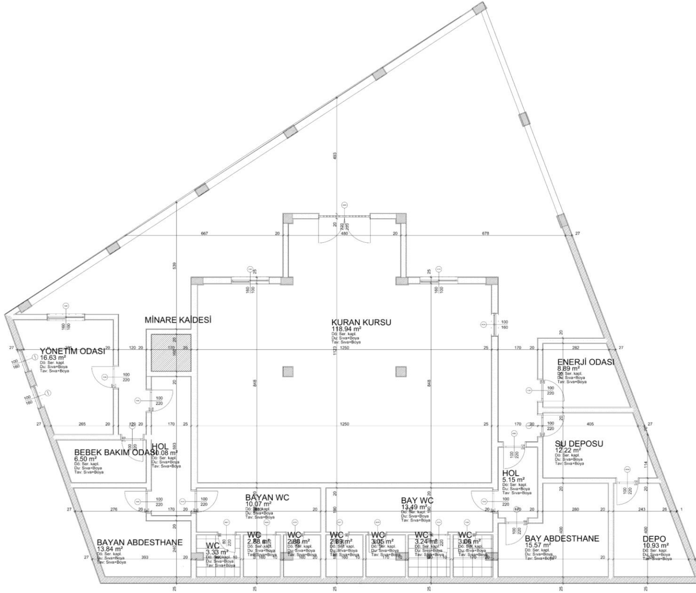
BODRUM KAT PLANI
