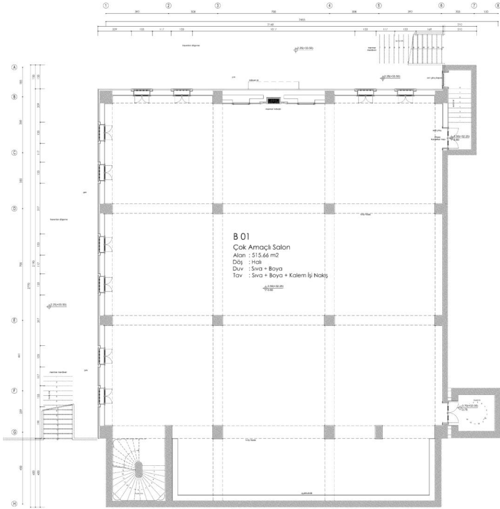
BODRUM KAT PLANI
