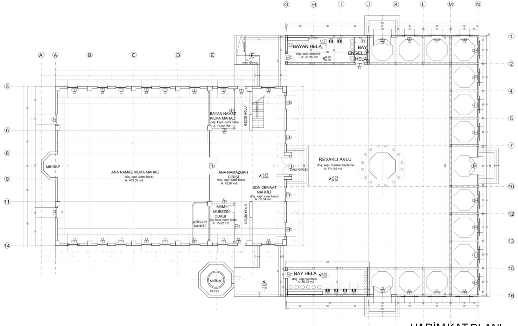
HARİM KAT PLANI
