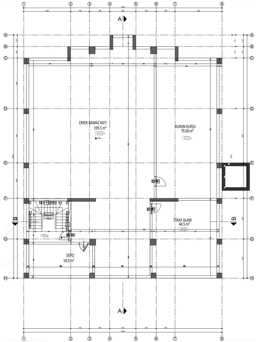
BODRUM KAT PLANI
