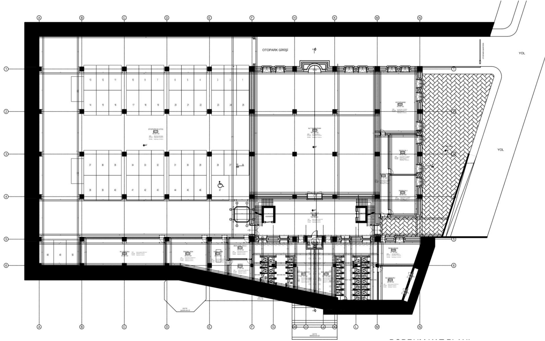
BODRUM KAT PLANI
