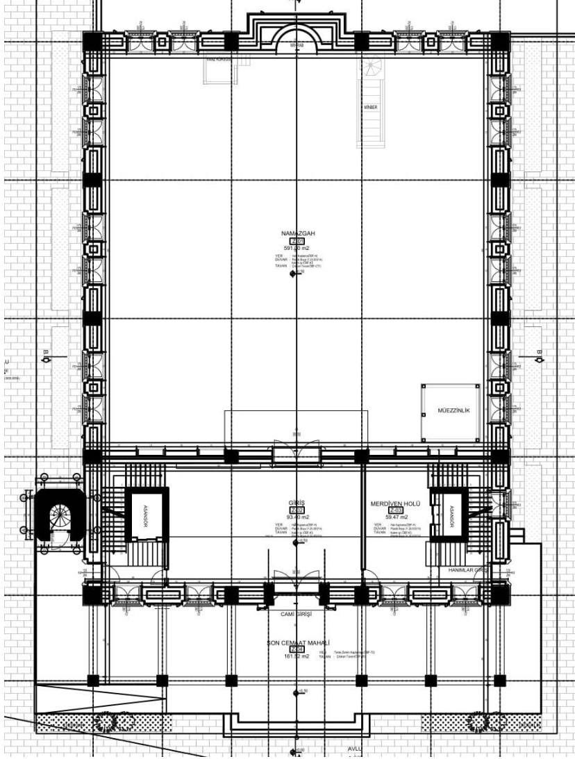
HARİM KAT PLANI
