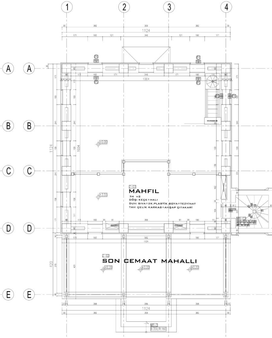
MAHFİL KAT PLANI
