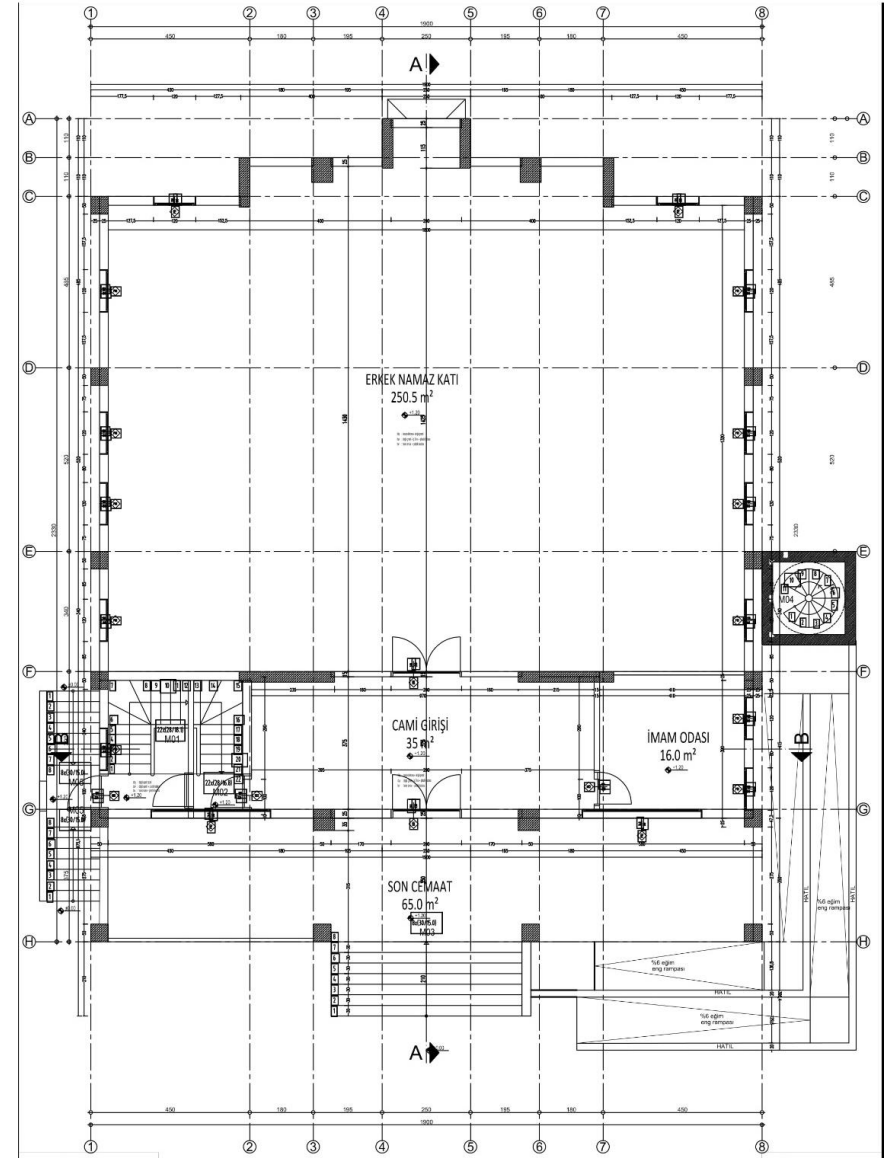
HARİM KAT PLANI
