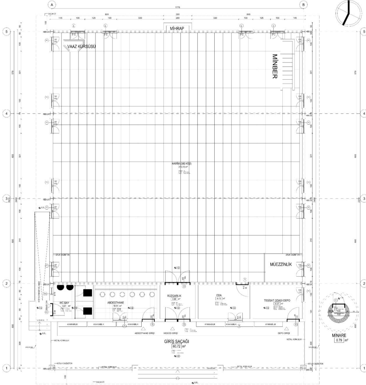
HARİM KAT PLANI
