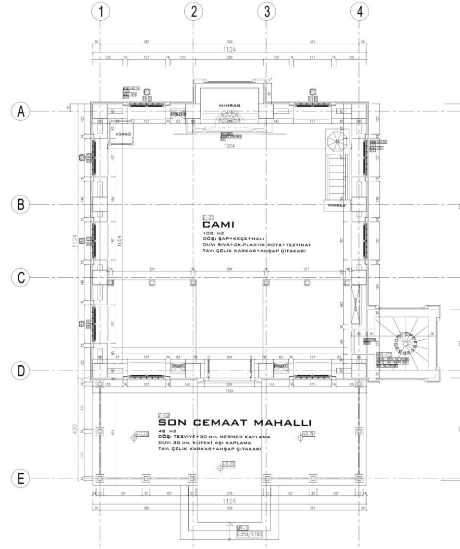
HARİM KAT PLANI
