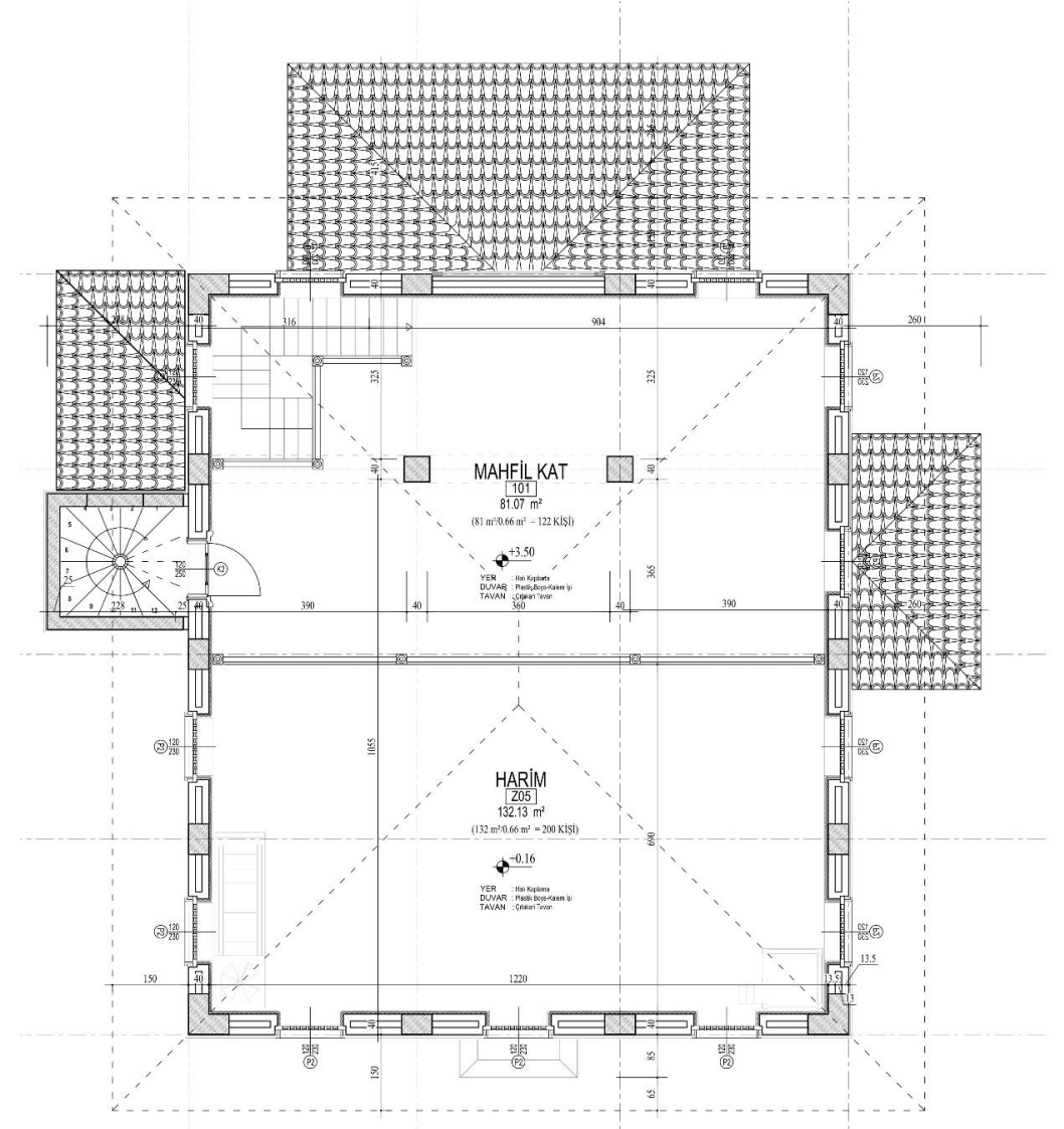
MAHFİL KAT PLANI
