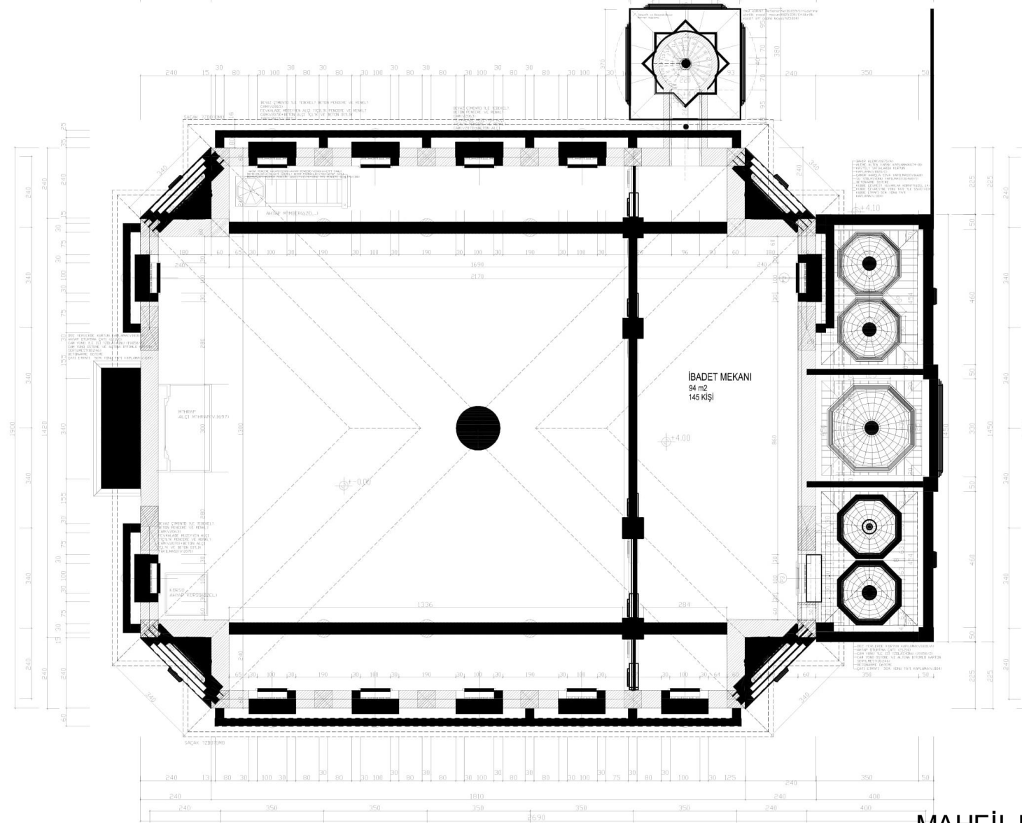
MAHFİL KAT PLANI
