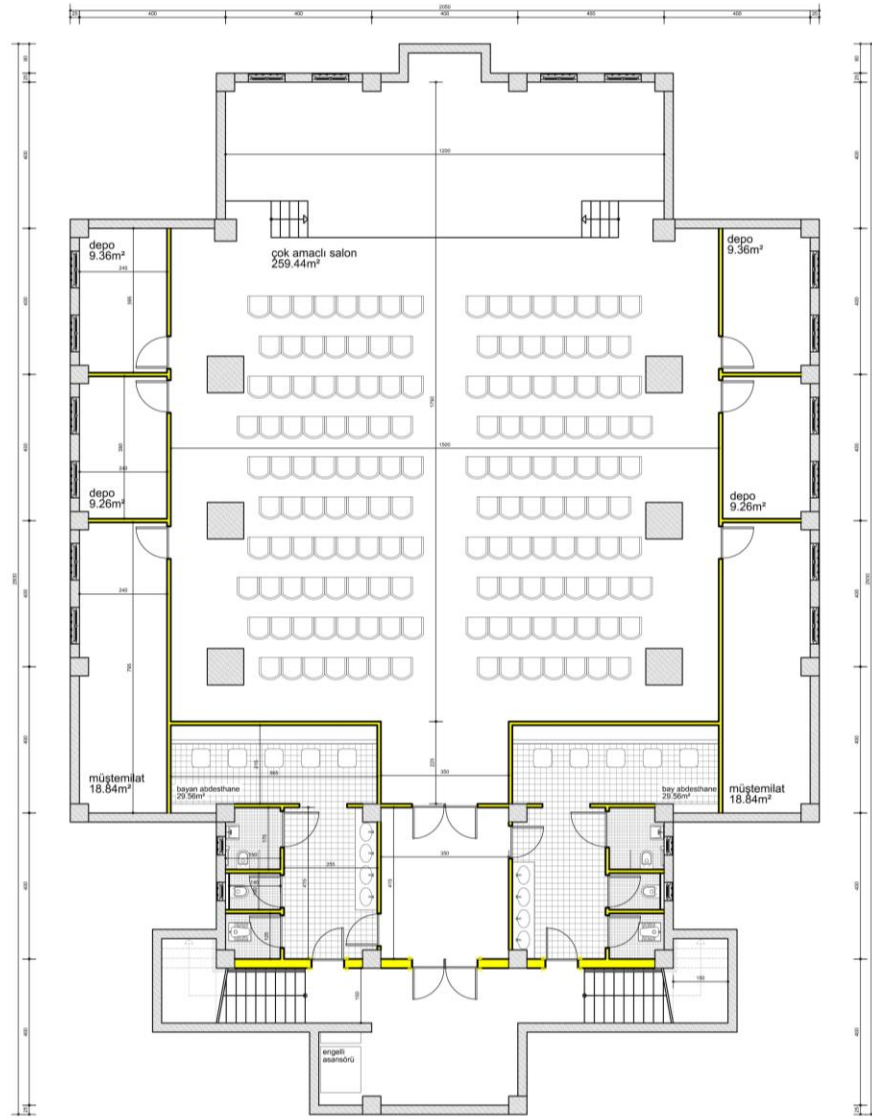
BODRUM KAT PLANI
