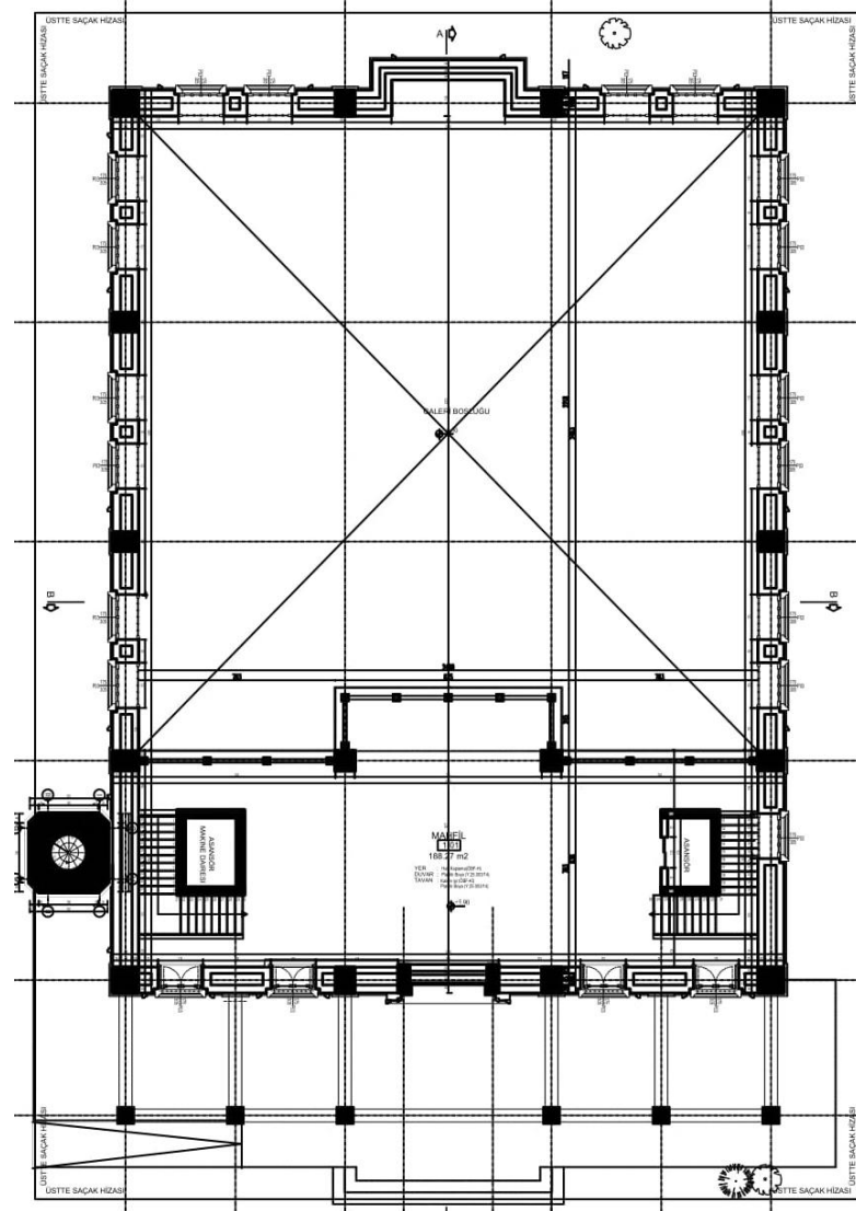
MAHFİL KAT PLANI
