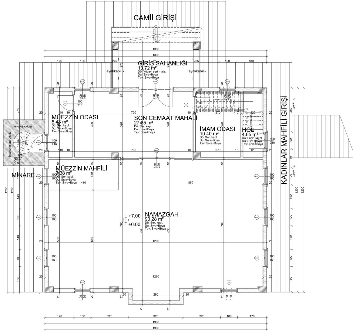
HARİM KAT PLANI
