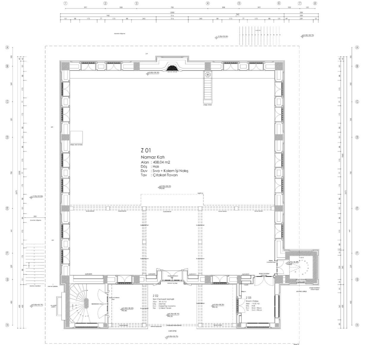
HARİM KAT PLANI
