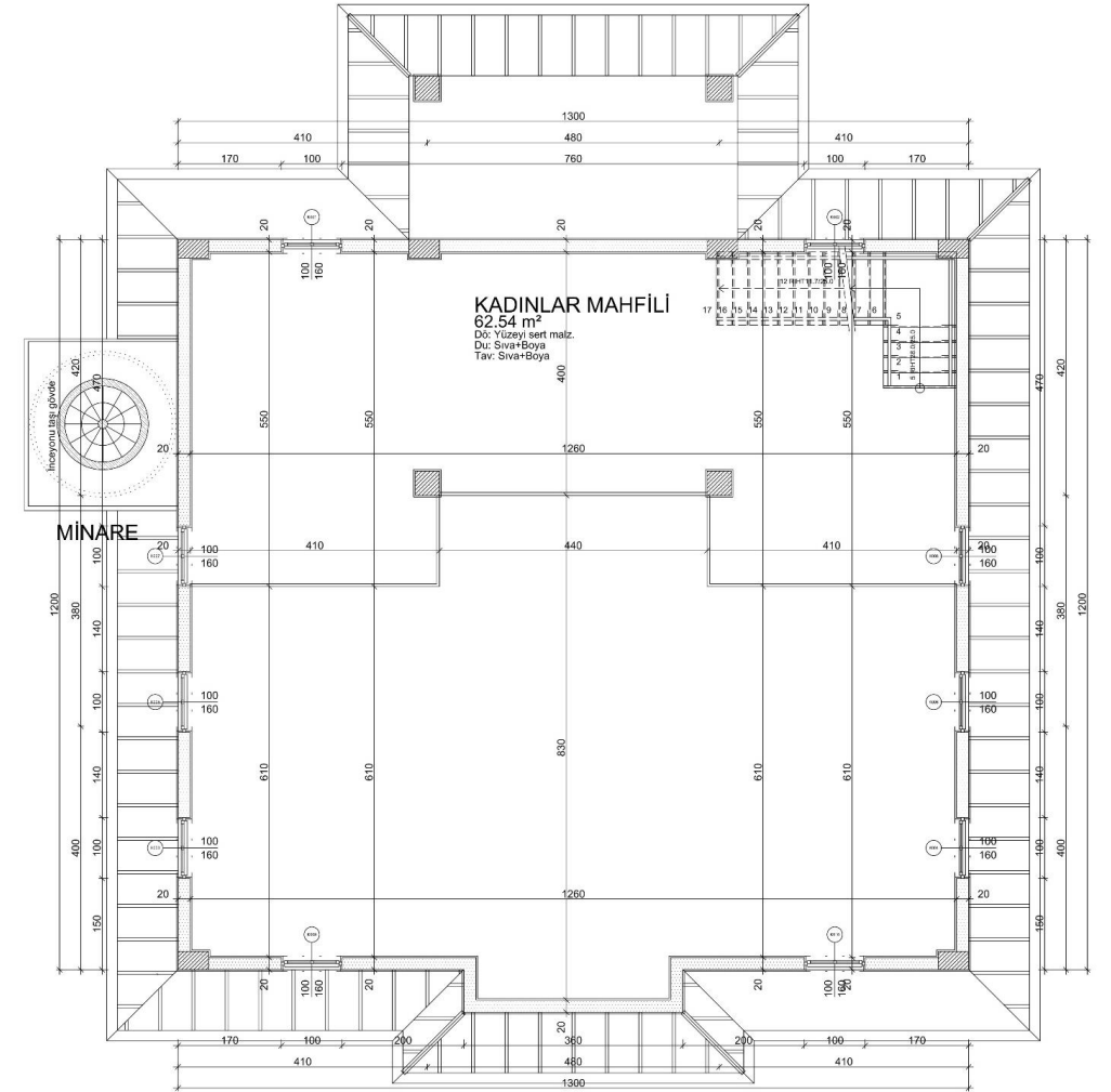
MAHFİL KAT PLANI
