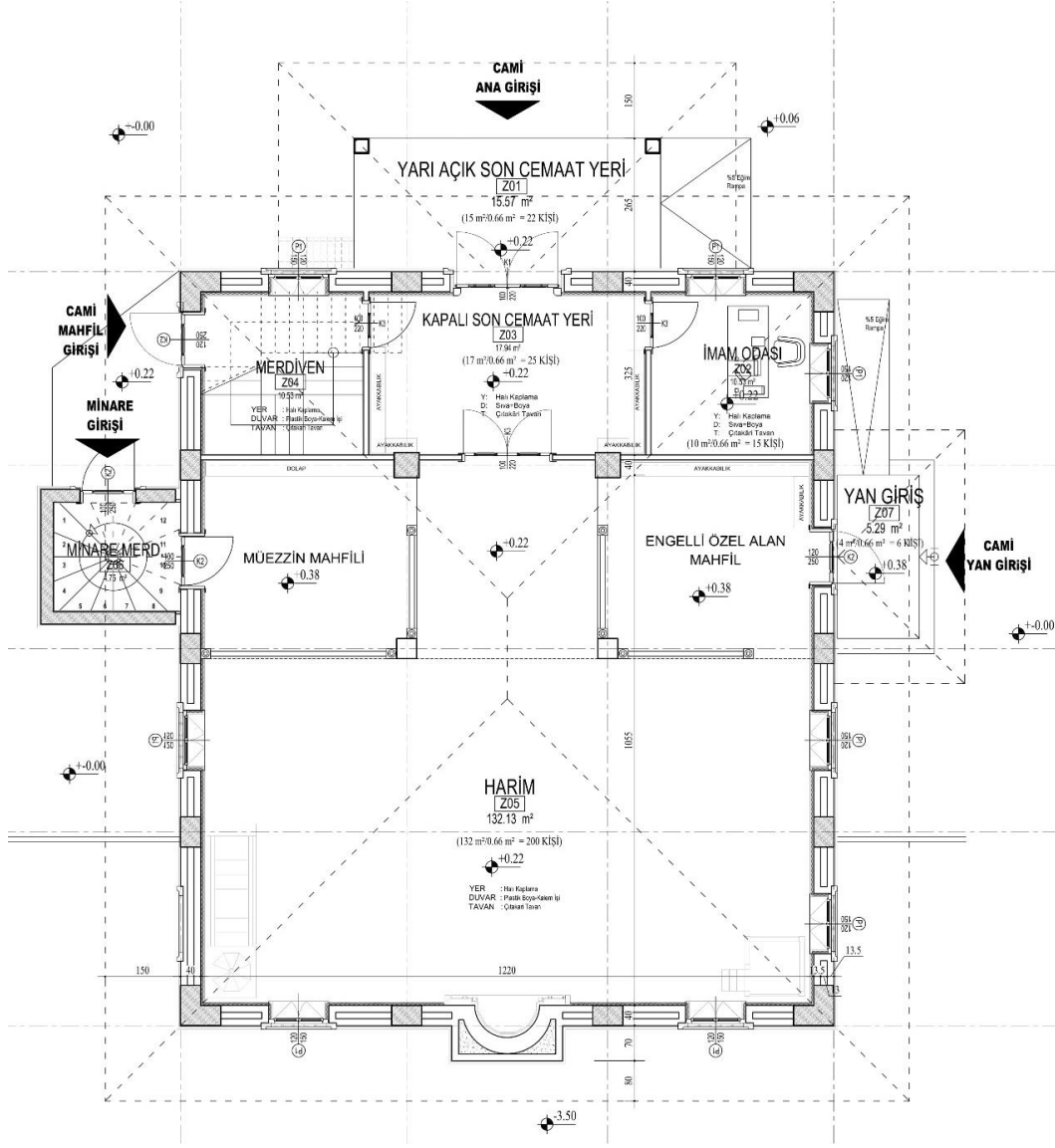
HARİM KAT PLANI
